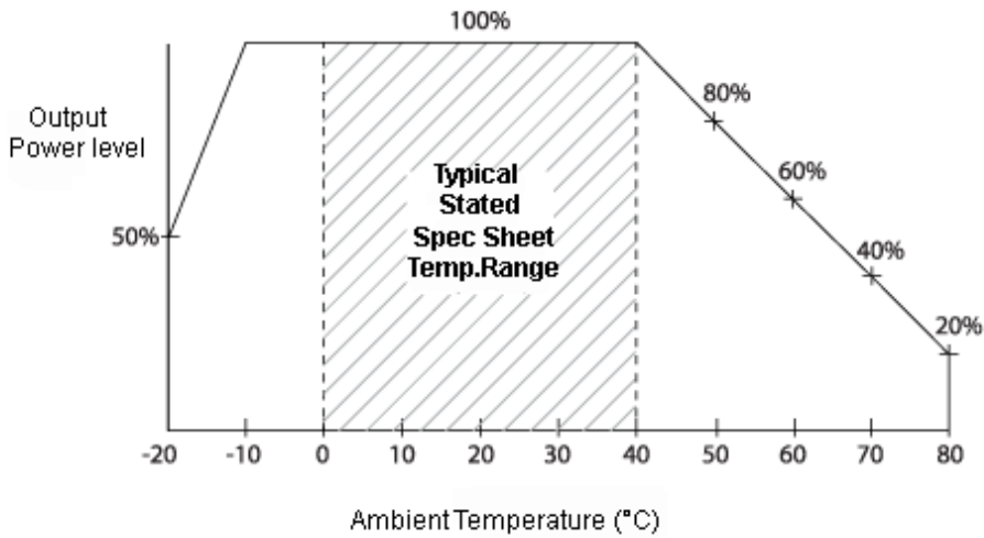
Typical External Power Supply Derating Curve (for Efficiency Level V and Level VI Products)
